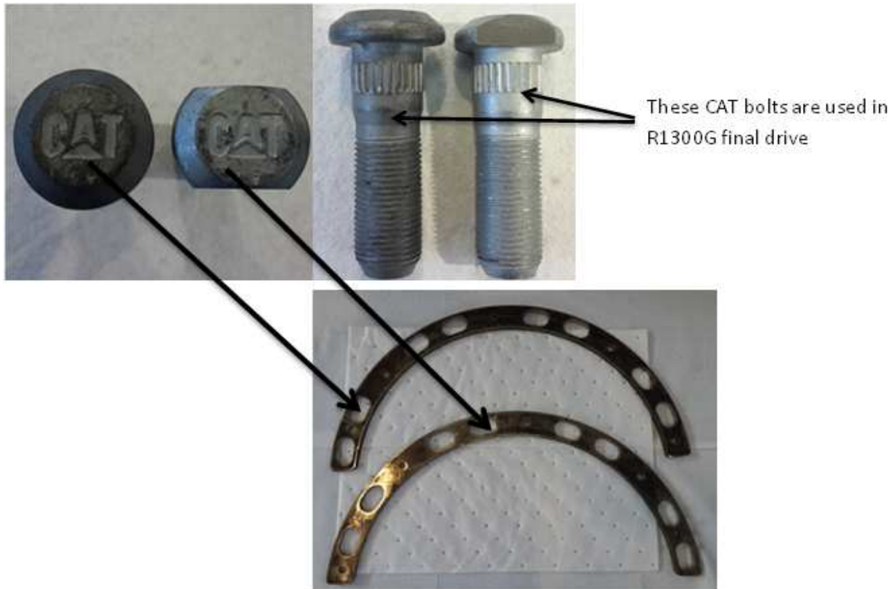
Semi-rings with locking holes for R1300G Final Drive Bolts (P/N 308-9259).
